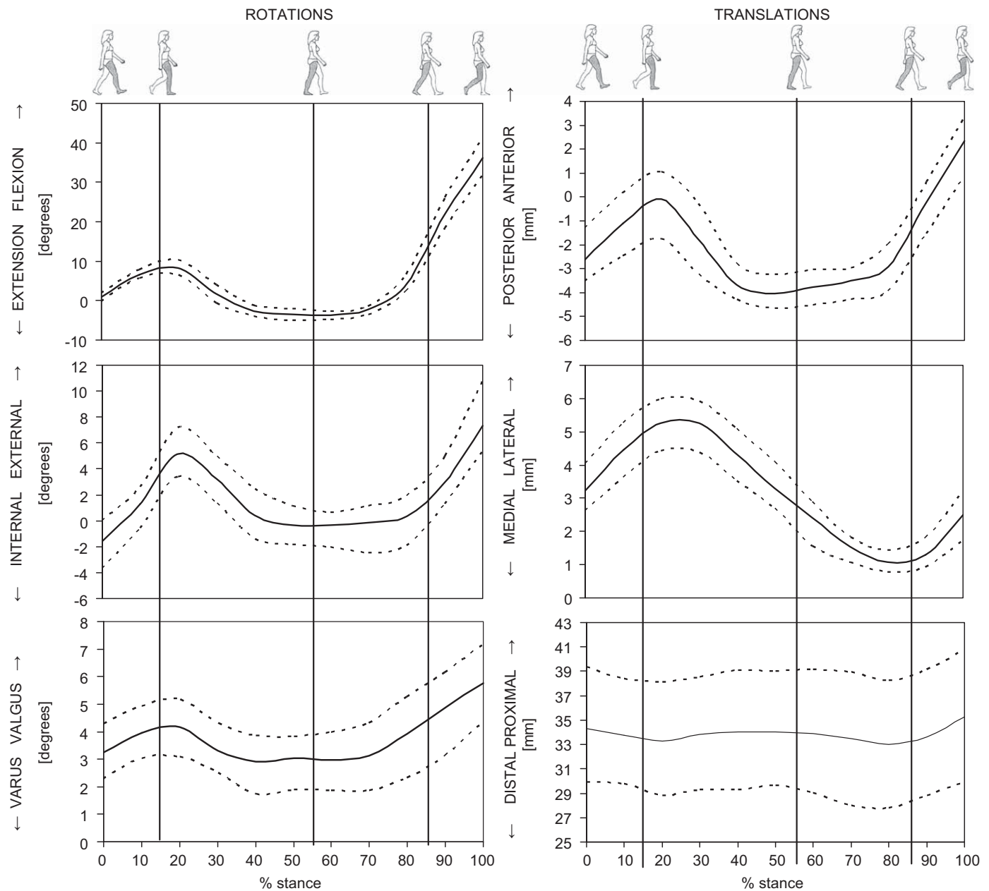
Fig. 4. Showing the 6DOF tibiofemoral kinematics of the knee joint measured during the stance phase of treadmill gait. The kinematics reported here represents the motion of femur relative to tibia. Solid lines represent contralateral toe-off, ipsilateral heelrise and contralateral heel-strike, respectively. The dashed lines denote the kinematic range: maximal and minimal displacement. The intervals between the solid lines represent loading response, midstance, terminal extension and pre-swing, respectively.
