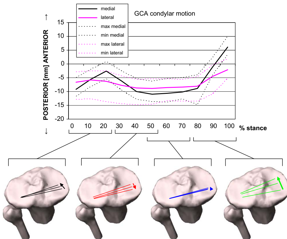
Fig. 6. Excursions of the medial and lateral condyles of the femur during stance phase determined in the anteroposterior direction. Geometrical center axis (GCA) of the femur was constructed for this measurement and the condylar centers were followed throughout the stance phase. Again, the medial femoral condyle was more mobile than the lateral.
