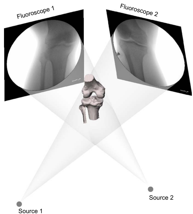
Fig. 2. Virtual reproduction of the fluoroscopic setup and tibiofemoral kinematics. The 3D MR-based models of the femur and tibia were matched to their projections on the fluoroscopic images.
